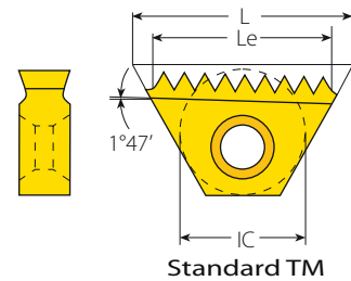
Standard TM
